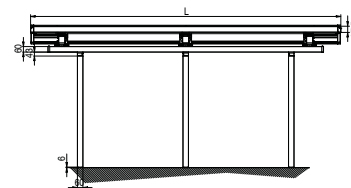
Vista frontale (3 profili guida) Frontal view (3 guide profiles)
