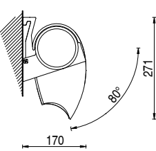
Installation façade 80°
