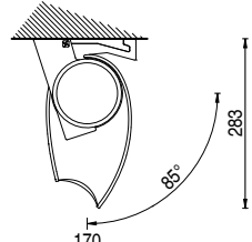
Installation plafond 85°
