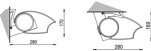
Installation façade
