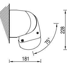
Installation façade 75°
