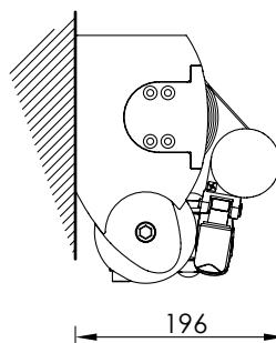
Montaggio a parete Wall installation
