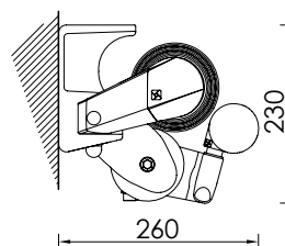
Montaggio a parete Wall installation
